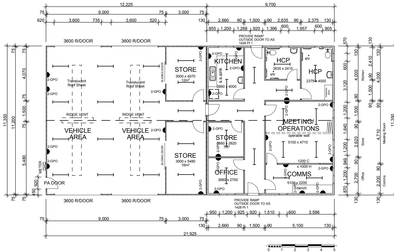
INDICATIVE METAL CLAD OPTION
